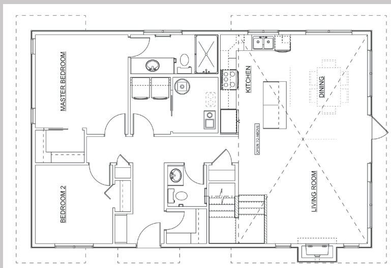
Main Floor - 1,241 SQ.FT.
